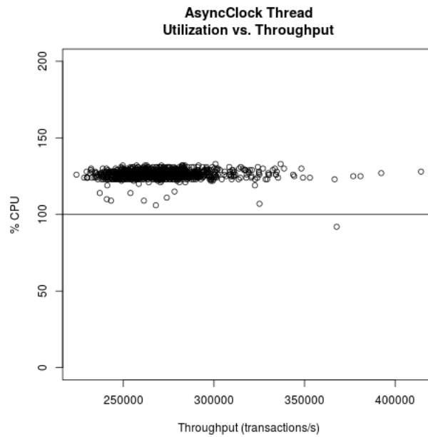
Figure 6.6: AsyncClock Thread Utilization vs. Throughput
